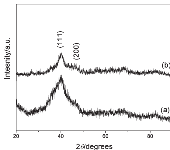
Figure 4. XRD patterns of (a) \text{FePt} and (b) \text{Fe}_4\text{Pt} alloy NPs synthesized by the thermal decomposition of [\text{NMe}_3\text{CH}_2\text{Ph}]_2[\text{Fe}_3\text{Pt}_3(\text{CO})_{15}] and [\text{NMe}_3\text{CH}_2\text{Ph}]_2[\text{Fe}_4\text{Pt}(\text{CO})_{16}] , respectively.
